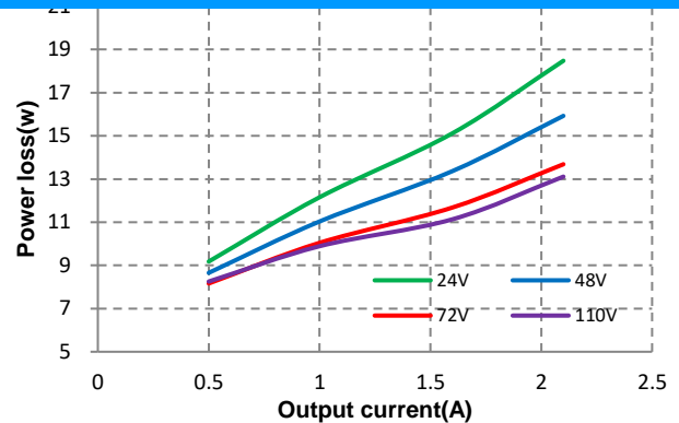
Figure 20: Power loss vs. load current at 25°C
