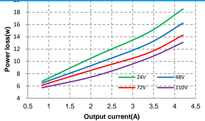
Figure 14: Power loss vs. load current at 25°C.
