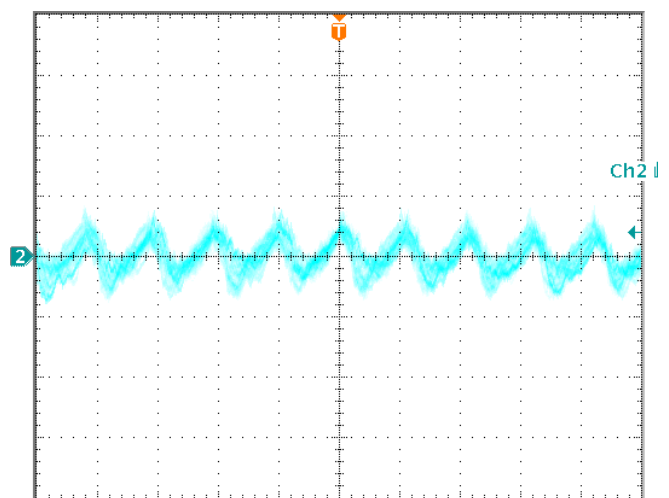
Figure 24: Output voltage ripple at V_{in}=72V and full load Trace: Vout: 25 mV/div, 2 \mu s /div; Bandwidth: 20 MHz.
