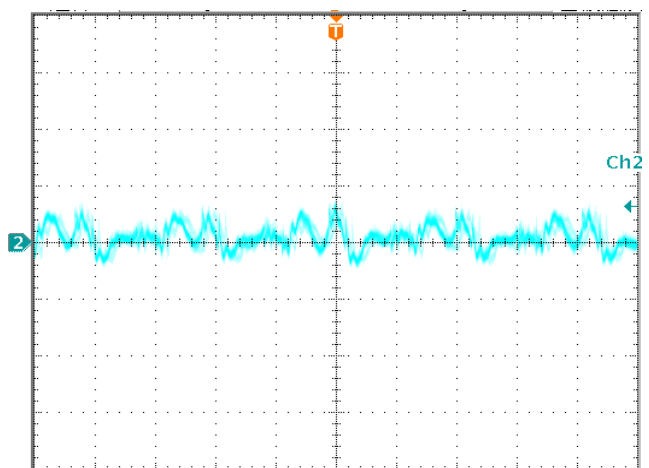
Figure 18: Output voltage ripple at V_{in}=72V and full load. Trace: Vout; 10 mV/div, 2μs/div; Bandwidth: 20 MHz.
