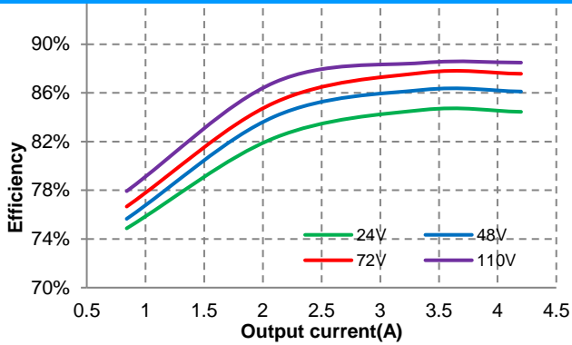
Figure 13: Efficiency vs. load current at 25°C.
