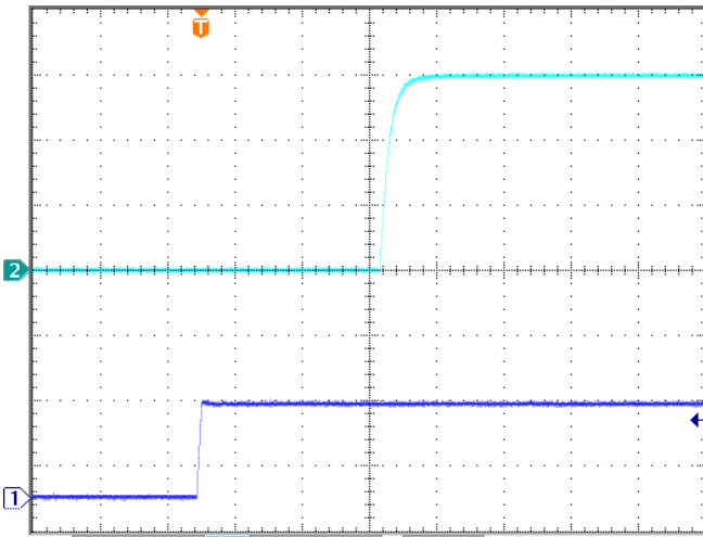
Figure 15: Turn-on transient at full load current (200ms/div). Top Trace: Vout, 8V/div; Bottom Trace: Vin, 50V/div
